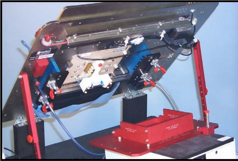
Backside of handler Test head undocked
