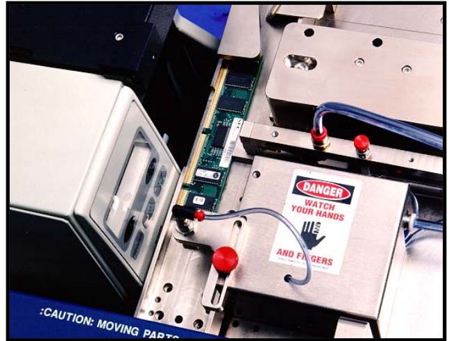
Pick & Place label applicator Eliminates ESD problems with direct peel label application methods
