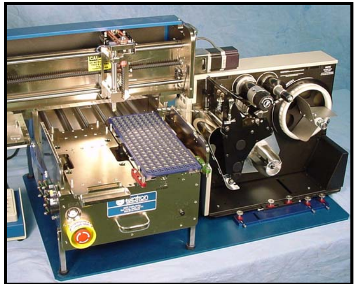
Pick & Place label applicator Eliminates ESD problems with direct peel label application methods
