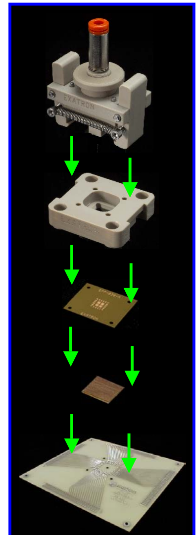
Top Loader Socket assembly
